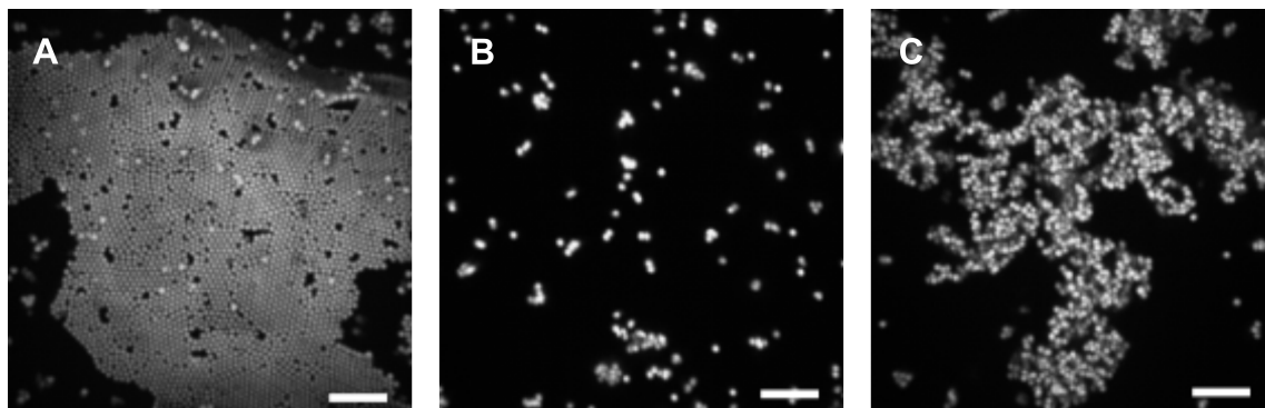
Figure 5.6: Comparison between aggregation of DNA-coated colloids and colloids surrounded by DNA free in solution. A: \lambda -DNA coated colloids aggregate into a flying colloidal carpet. B: Colloids surrounded by a solution of \lambda -DNA ( \lambda -DNA is present at the same concentration as used in figure A) hardly aggregate; only small 3D clusters appear. C: If the concentration of \lambda -DNA is increased 100x, more aggregation is visible. In contrast to figure A this leads to 3D branches rather than 2D carpets. All scale bars are 10 \mu\text{m} .
