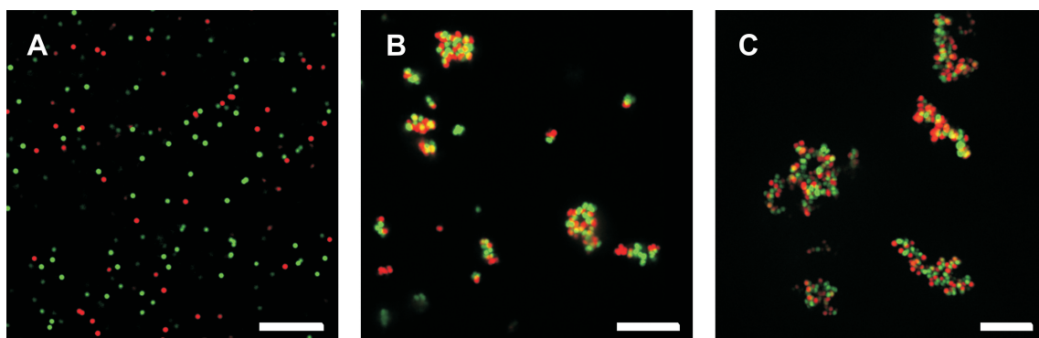
Figure 3.1: Confocal images of the clusters taken at different time points. A: 30 min after mixing - at this stage only monomers, dimers and trimers are present. B: several hours after mixing - multiple colloid clusters start to appear surrounded by dimers and trimers. C: 1 day after mixing - the clusters have reached their final stage and all dimers and trimers have disappeared. All scale bars indicate 10\ \mu m .
