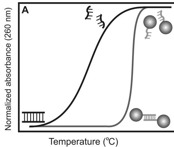
Figure A.1: Schematic representation of the dissociation curve of free DNA in solution compared to the dissociation curve of DNA grafted to colloids. Note that the same DNA has a much narrower melting curve once grafted to colloids. Also the melting temperature shifts toward higher temperatures for colloid bound DNA.
