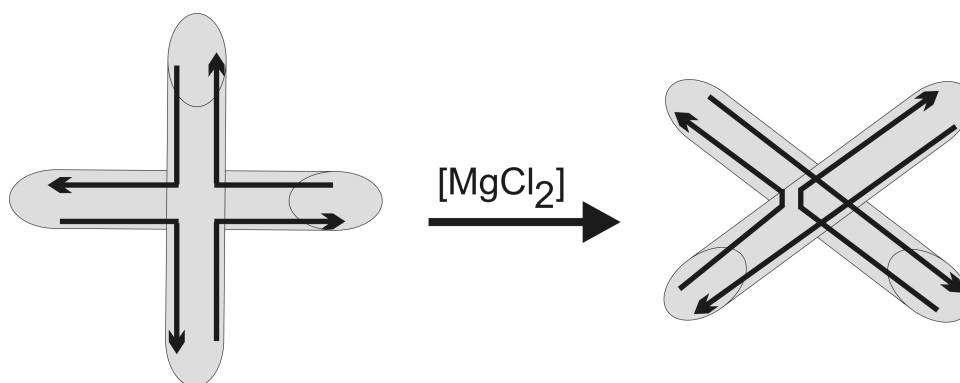
Figure 6.2: Illustration of the ion-dependent folding equilibrium of the four-way DNA junction. At low salt concentrations the junction exists in an extended, unstacked conformation. Upon addition of divalent metal ions, such as magnesium ions, the junction folds into the stacked X-structure [162]
