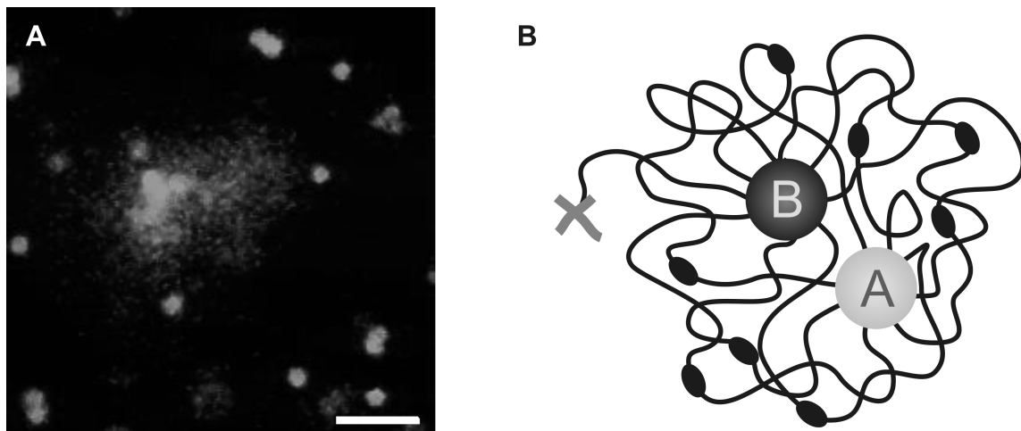
Figure 3.4: DNA gets expelled from the gap between two neighboring colloids. A: Non fluorescent colloids grafted with YOYO stained \lambda -DNA. Scale bar is 10\ \mu\text{m} . B: Cartoon of \lambda -DNA coated colloids. DNA is long enough to stretch over neighboring colloids. No free ends have to be present for dimers or bigger assemblies.
