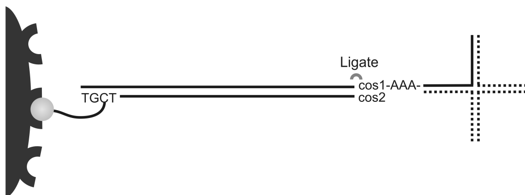
Figure 6.7: DNA construct used to string four colloids together with a DNA-junction. A fragment of the pBelo-DNA is restricted at two sides. One carries a cos2-end, which can be used to attach the junction overhang (the AAA nucleotides are added for more flexibility). The opposite end contains a 4-base overhang. This is filled in with 4 nucleotides (TGCT); one labeled with a biotin-tag (dCTP). For clarity the eventual junction is depicted with dotted lines.
